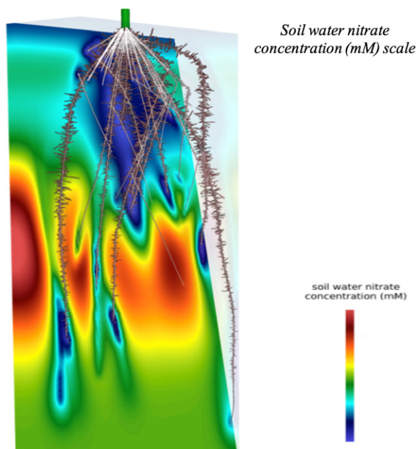
Figure 2. SimRoot image of maize root system dynamically interacting with a nitrate-leaching pulse.
