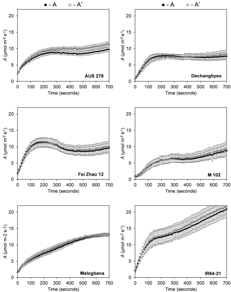
Fig. 5. The response of uncorrected leaf CO 2 assimilation (A; filled circles) and the response of leaf CO 2 assimilation corrected for stomatal limitation (A*; open circles) over time in flag leaves of six rice accessions. The first line at 100 s indicates the mean time for the activation of Rubisco ( \tau ) per accession. Each point represents the mean of at least six plants \pm SE ( n=6-8 ).
